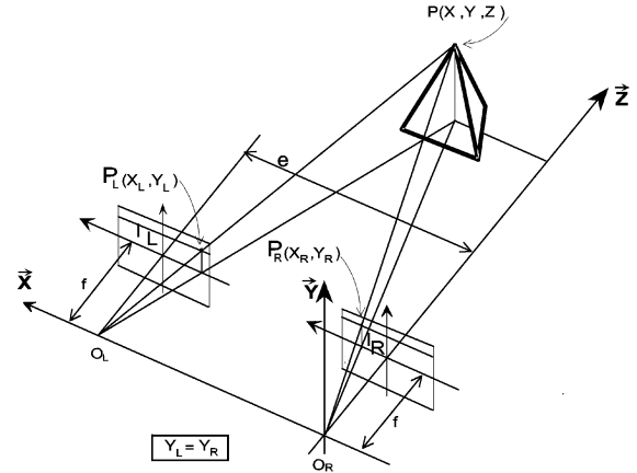
Fig. 1. Configuration of the stereo vision system.
