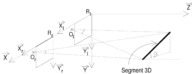
Fig. 6. Inclination angle \beta of a 3-D segment.
