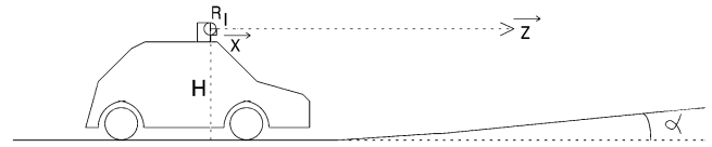
Fig. 4. Inclination angle \alpha of the road plane and height H of the stereo vision system.
