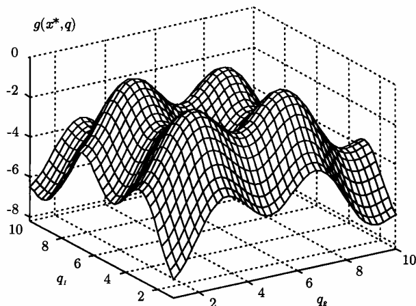
Figure 6. Shape of the constraint function g(x^*, q) for problem 3.
