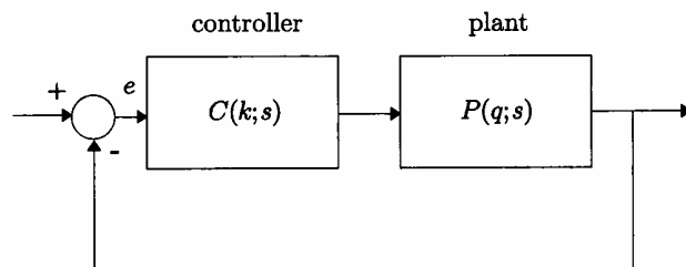
Figure 7. Control scheme.
