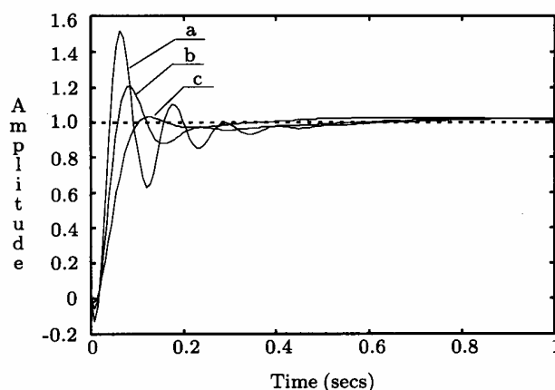
Figure 8. Optimal step responses of the closed-loop system.
