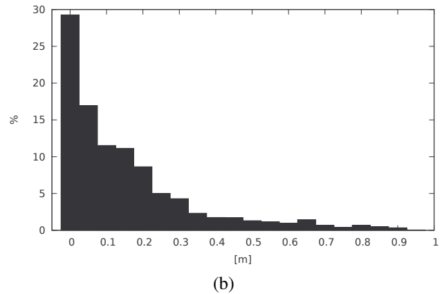
Fig. 7. Plot of lateral crosstrack error (a) and relative histogram (b) during the experiment of 21 minutes of autonomous operations in urban and rural environments with vehicle in autonomous Leader Vehicle following.
