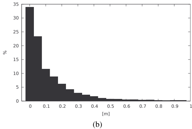
Fig. 6. Plot of lateral crosstrack error (a) and relative histogram (b) during the experiment of 22 minutes of autonomous operations on campus with autonomous GPS Waypoint following.
