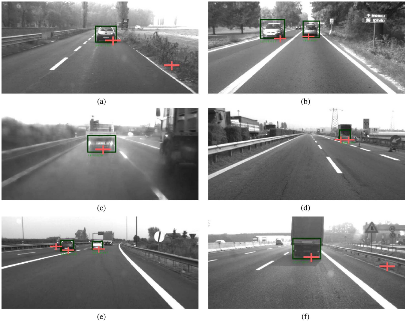
Fig. 18. Examples of correct results. (a) The algorithm works reliably in simple cases. (b) It detects both vehicles moving away and approaching. It works even in hard cases, such as (c) rainy and (d) noisy scenarios (note the double radar detection). It can detect (e) multiple cars and (f) trucks.
